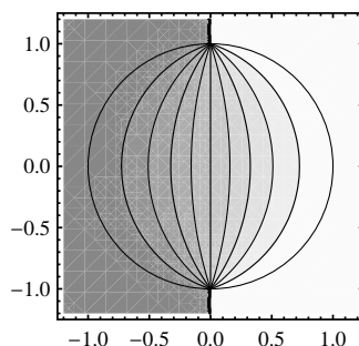
Figure 5: A harmonic function on the unit disc.
